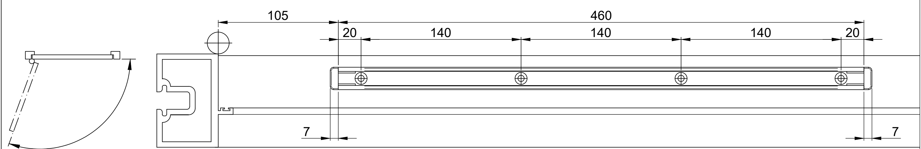
"A-A" RS.11000 - 348 Connecting Bar - Micro Rail - Profile Frame
